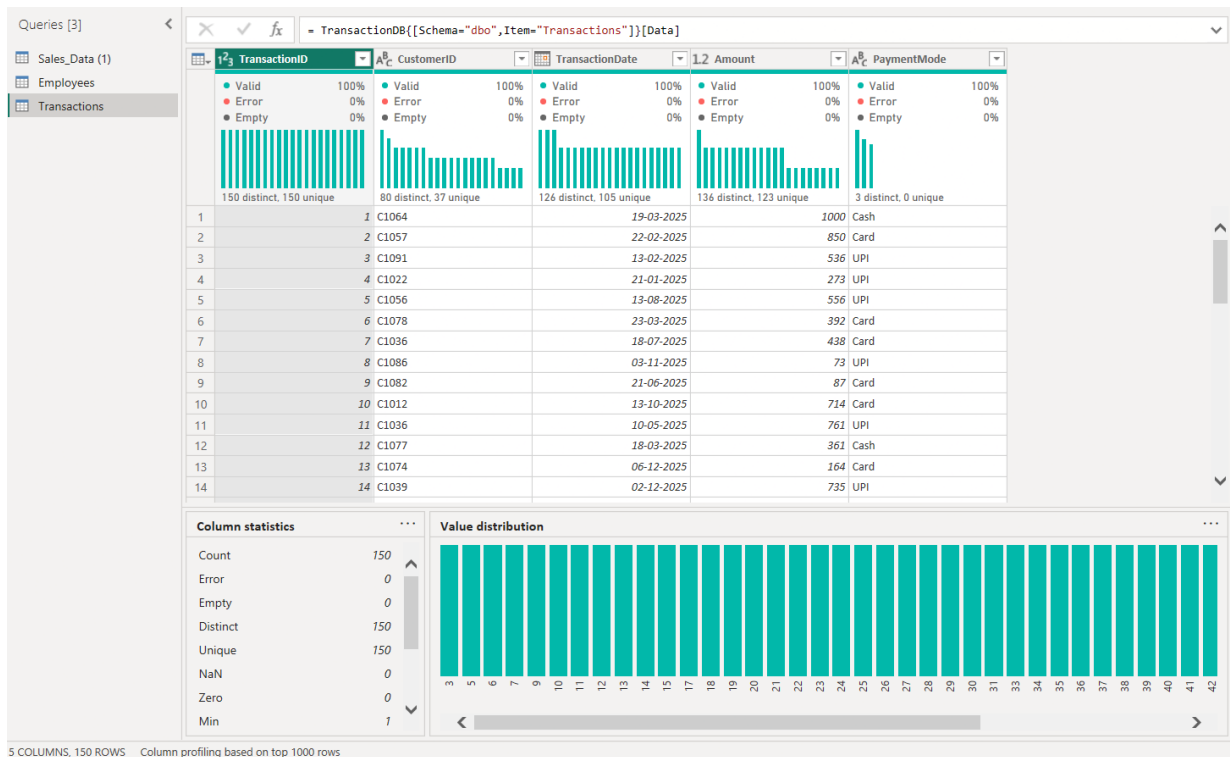
Figure 4: Transactions dataset profiling showing distinct/unique counts and column statistics.
